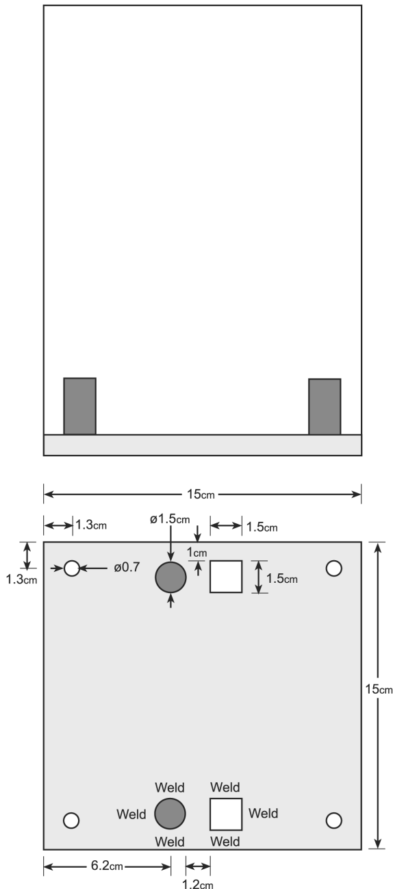
Target Base (plan view)
